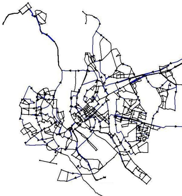
Fig. 7. Suggested DMA distribution at Riga water distribution network. Sensor installation sites shown in blue.
