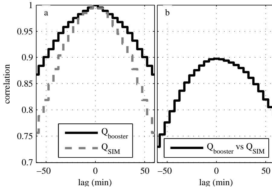
Fig. 6. (a) Auto-correlation of Q_{\text{booster}} and Q_{\text{SIM}} and (b) cross-correlation between Q_{\text{booster}} and Q_{\text{SIM}} for different time lags on a 5-min time scale.
