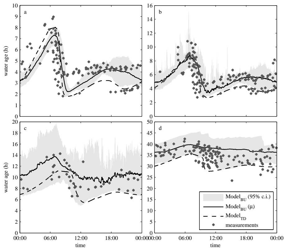
Fig. 8. Measured and modelled water age at location (a) 1; (b) 2; (c) 3 and (d) 4. N.B. the 95% confidence interval is due to variation, not to uncertainty.
