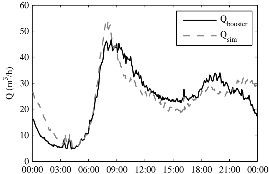
Fig. 5. Measured and simulated flows on a 5-min time scale.
