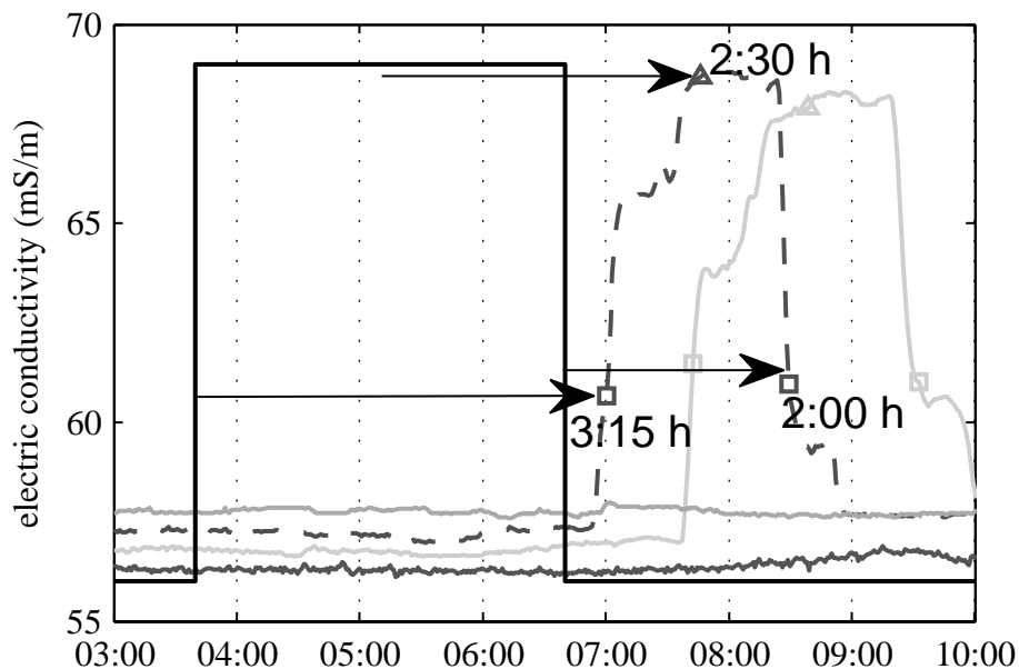
Fig. 3. Reconstructed EC at booster locations and measured EC at locations 1 and 2 (Wednesday, 3 September 2008) plus associated travel times.
