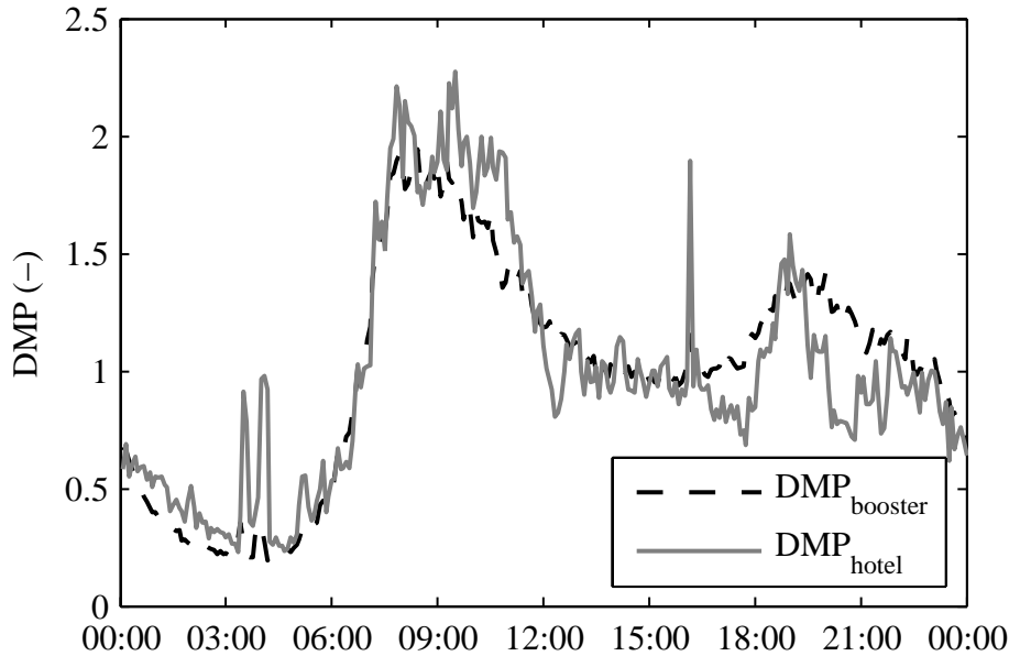
Fig. 4. Demand multiplier patterns as used in the Model TD and Model BU .
