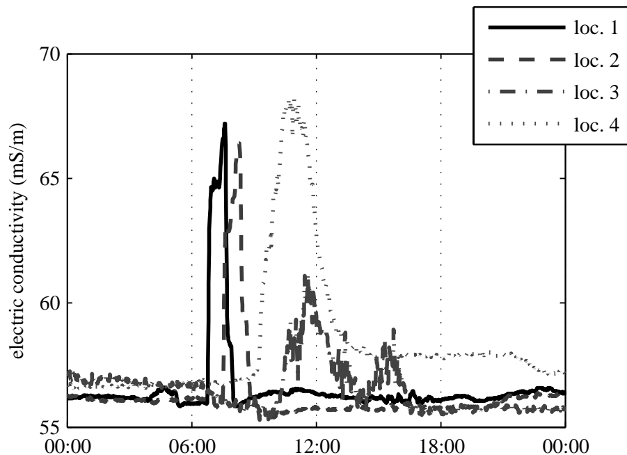
Fig. 7. Measured EC at locations 1–4 at Thursday, 4 September 2008. N.B. EC at location 4 has 24 h delay.
