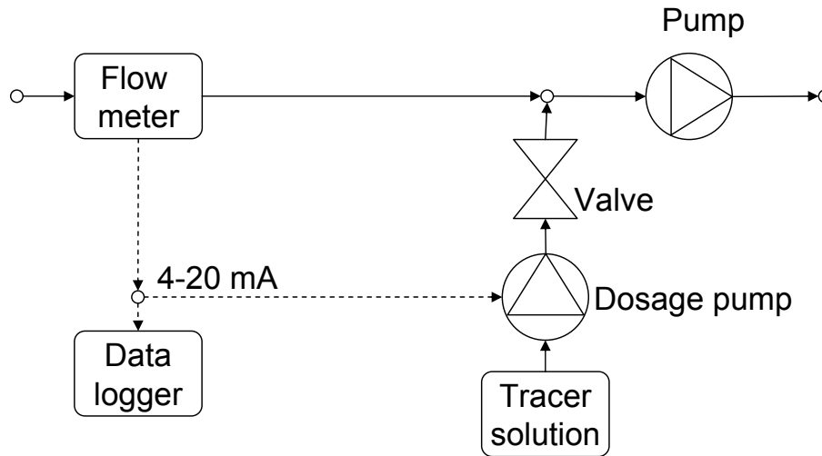
Fig. 2. Measurement setup for adding tracer solution.
